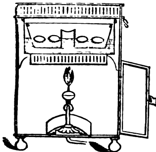
Fig. 21. - Transverse Section.
