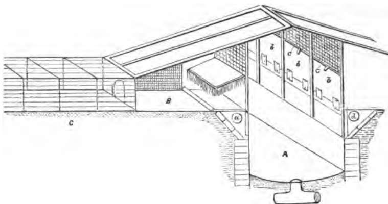
Fig. 16.—Artificial Rearing-home
